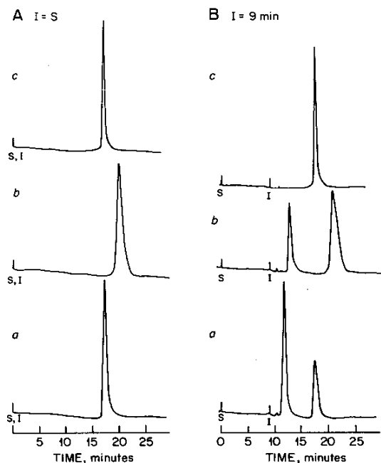
Fig. 7. Chromatographic behavior of \alpha -chymotrypsinogen as a function of organic modifier and injection time. A = Injection at the start of the gradient. B = Injection 9 min after the start of the gradient. Mobile phases: (a) 1-propanol-water (45:55, v/v); (b) 2-propanol-water (45:55, v/v); (c) acetonitrile-water (80:20, v/v). The overall concentration of H_3PO_4 in each mobile phase is 10 mM. Other conditions, see Fig. 2.
