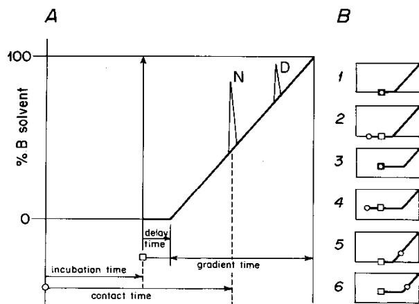
Fig. 1. Illustration of incubation experiments. (A) Definition of incubation, contact, delay and gradient times. (B) Illustration of various kinetic experiments of denaturation on the bonded phase surface. See text for details. ○, Injection time; □, start of the gradient.
