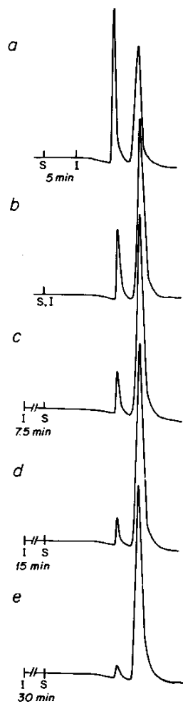
Fig. 5. Chromatographic behavior of lysozyme as a function of injection times relative to the start of the gradient. S = Start of gradient; I = injection time. Sample: 10 mg/ml lysozyme in mobile phase A, 5 \mu l injected. Other conditions: see Fig. 2. a = Injection 5 min after start of gradient. Incubation times: b = 0 min; c = 7.5 min; d = 15 min; e = 30 min.
