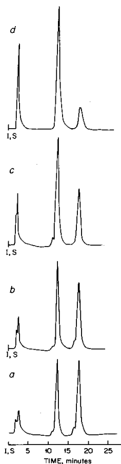
Fig. 3. Chromatographic behavior of papain with constant surface contact time as a function of the starting 1-propanol mobile phase concentration. a = Control, mobile phase A; b = 4% mobile phase B in A, i.e. 1.8% 1-propanol; c = 8% mobile phase B in A, i.e. 3.6% 1-propanol; d = 12% mobile phase B in A, i.e. 5.4% 1-propanol. Other conditions: see Fig. 2.
