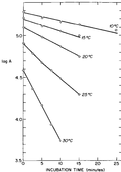
Fig. 6. First-order kinetic plots of the rate of denaturation of lysozyme at various column temperatures as a function of incubation time on the bonded phase surface. Log A = logarithmic area of the first (active) peak. Incubation solvent: 10 mM H_3PO_4 (pH 2.2). Other conditions: see Fig. 2.
